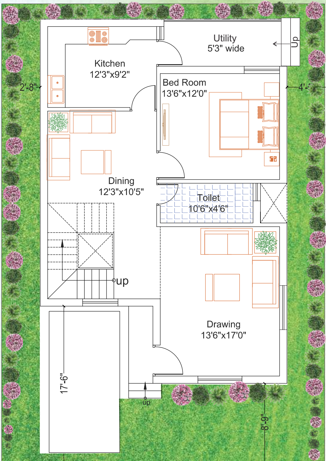
GROUND FLOOR PLAN Built Up Area :- 1040.00 sq.ft.
