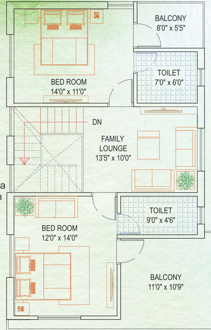
FIRST FLOOR PLAN Built Up Area :- 892.00 sq.ft.
