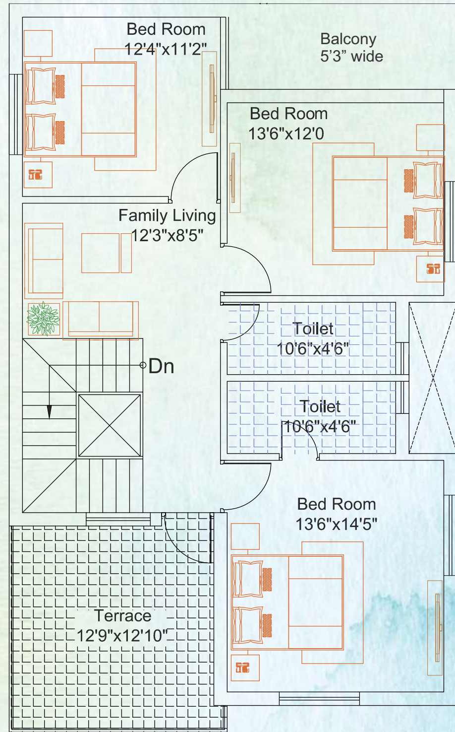
FIRST FLOOR PLAN Built Up Area :- 1240.00 sq.ft.
